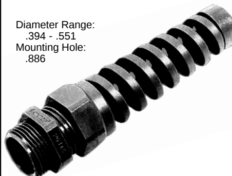
PG-16 PIGTAIL STRAIN RELIEF P/N 28184
